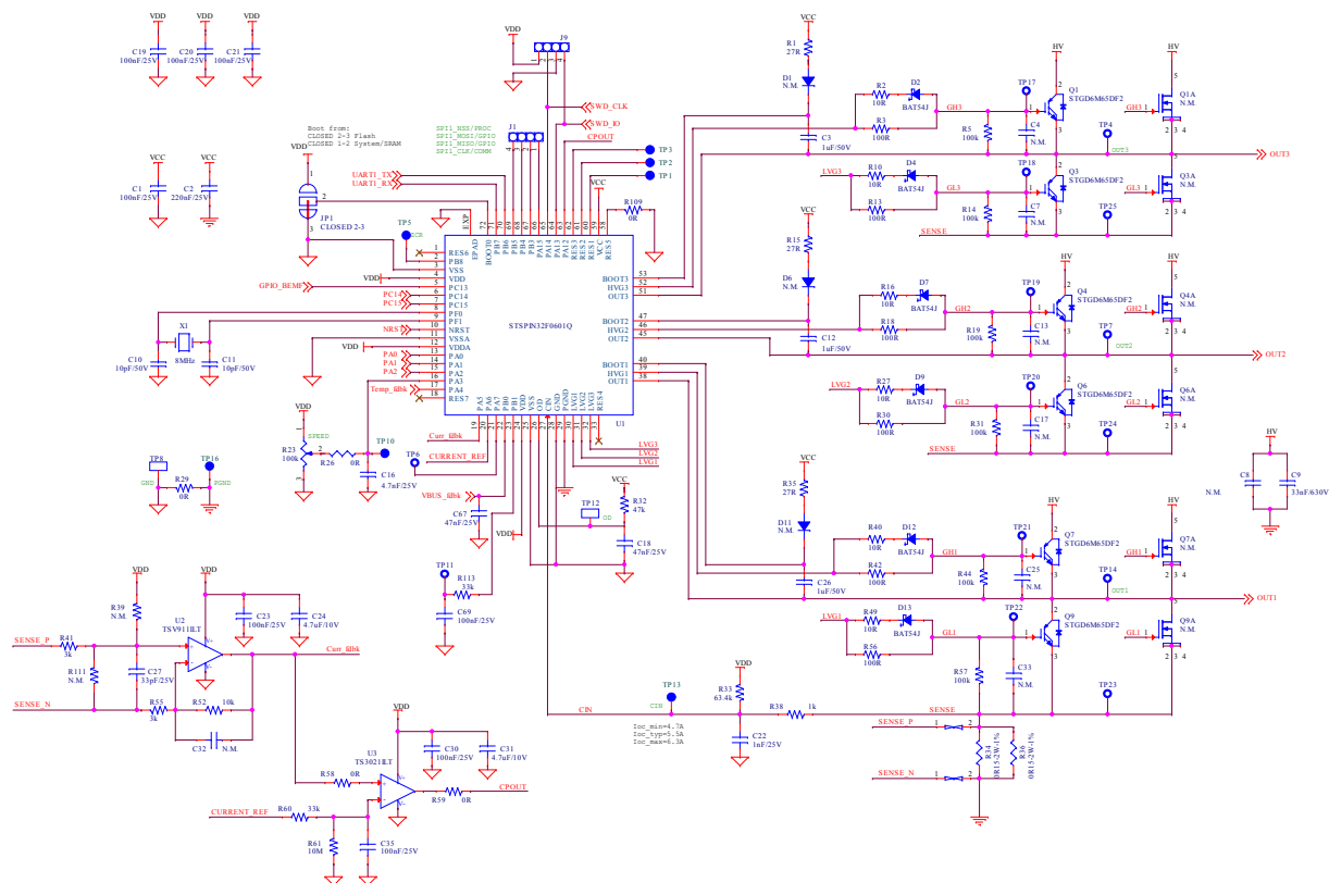
Figure 2. EVSPIN32F06Q1S1 schematic – Feedback network
