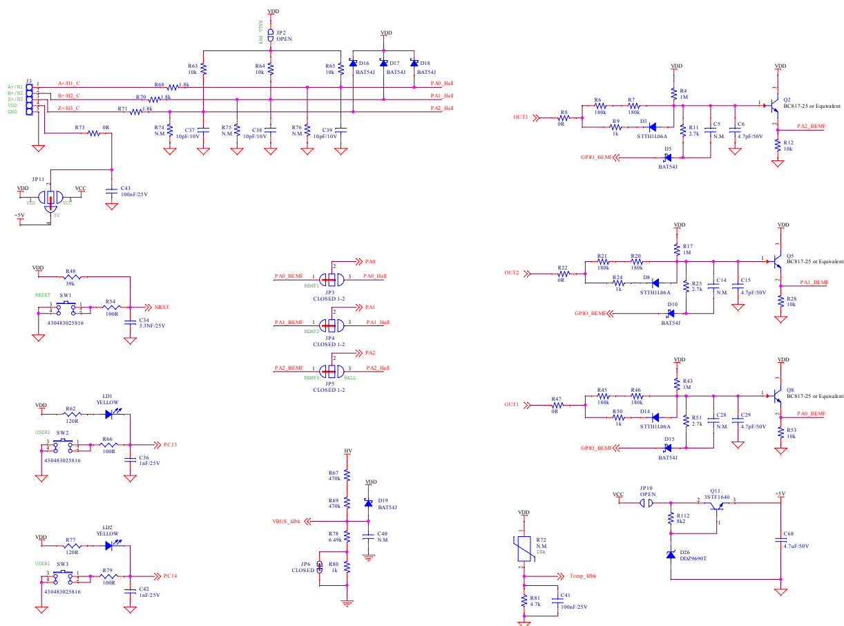
Figure 2. EVSPIN32F0601S1 schematic – Feedback network
