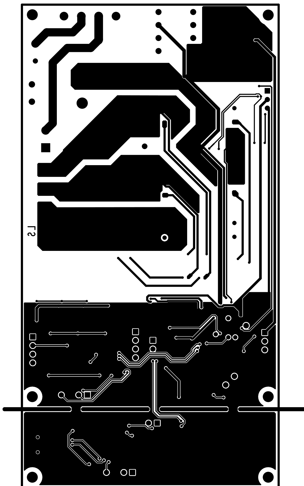
Figure 8. EVSPIN32F0601S1 – Layout (bottom layer)
