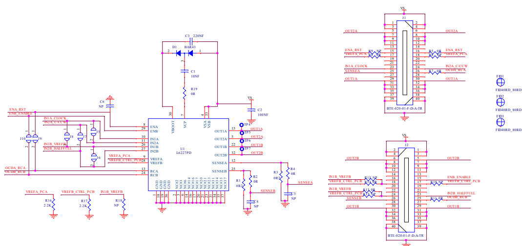
Figure 8. EVL6227-PLUG
