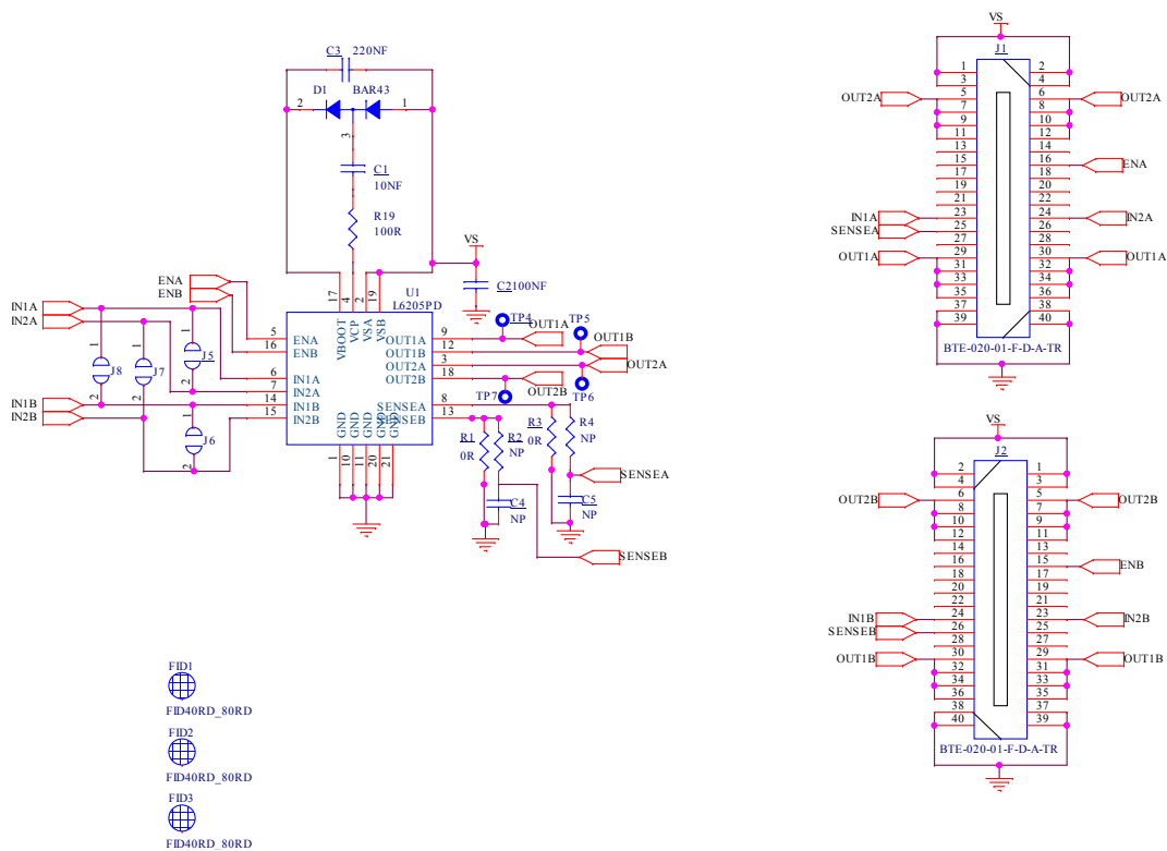
Figure 2. EVL6205-PLUG
