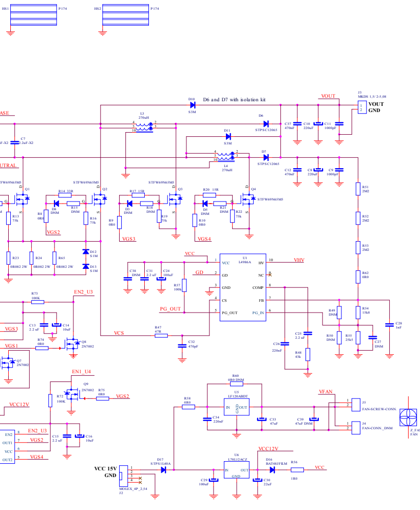
Figure 1. EVL4986A-1KWBL demo board schematic
