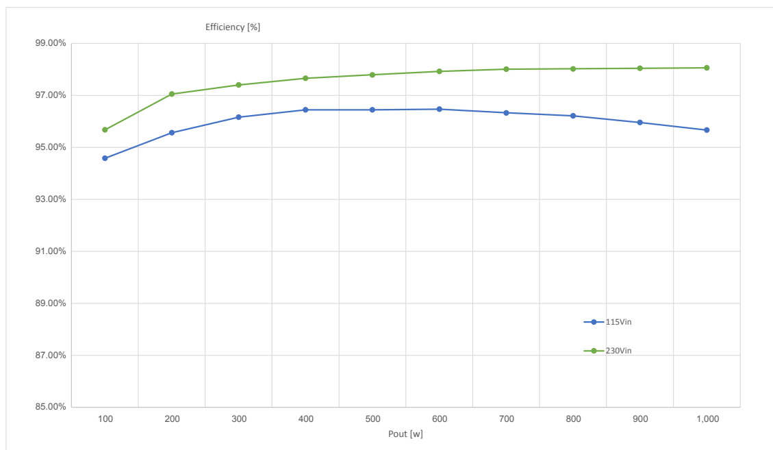
Figure 2. EVL4986A-1KWBL efficiency
