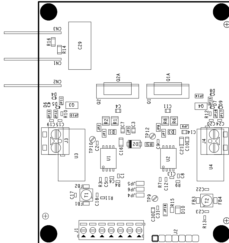
Figure 3. EVALSTGAP2SiCSC – Layout (component placement top view)
