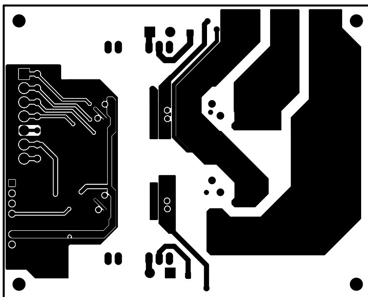
Figure 6. EVALSTGAP2HSM – Layout (bottom layer)
