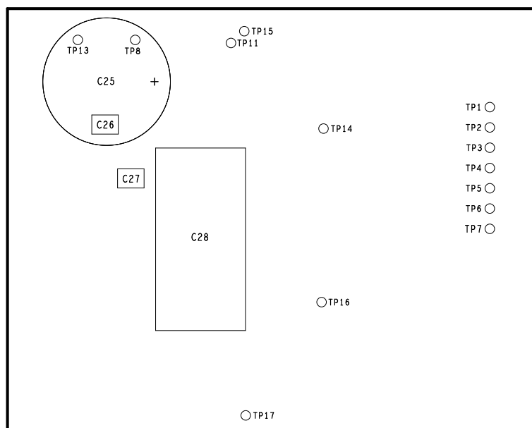
Figure 4. EVALSTGAP2HSCM – Layout (component placement bottom view)
