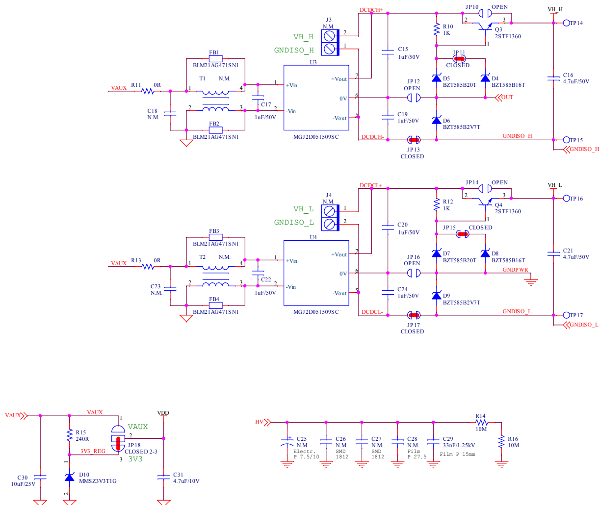
Figure 2. EVALSTGAP2HSCM circuit schematic – supply, connectors and decoupling
