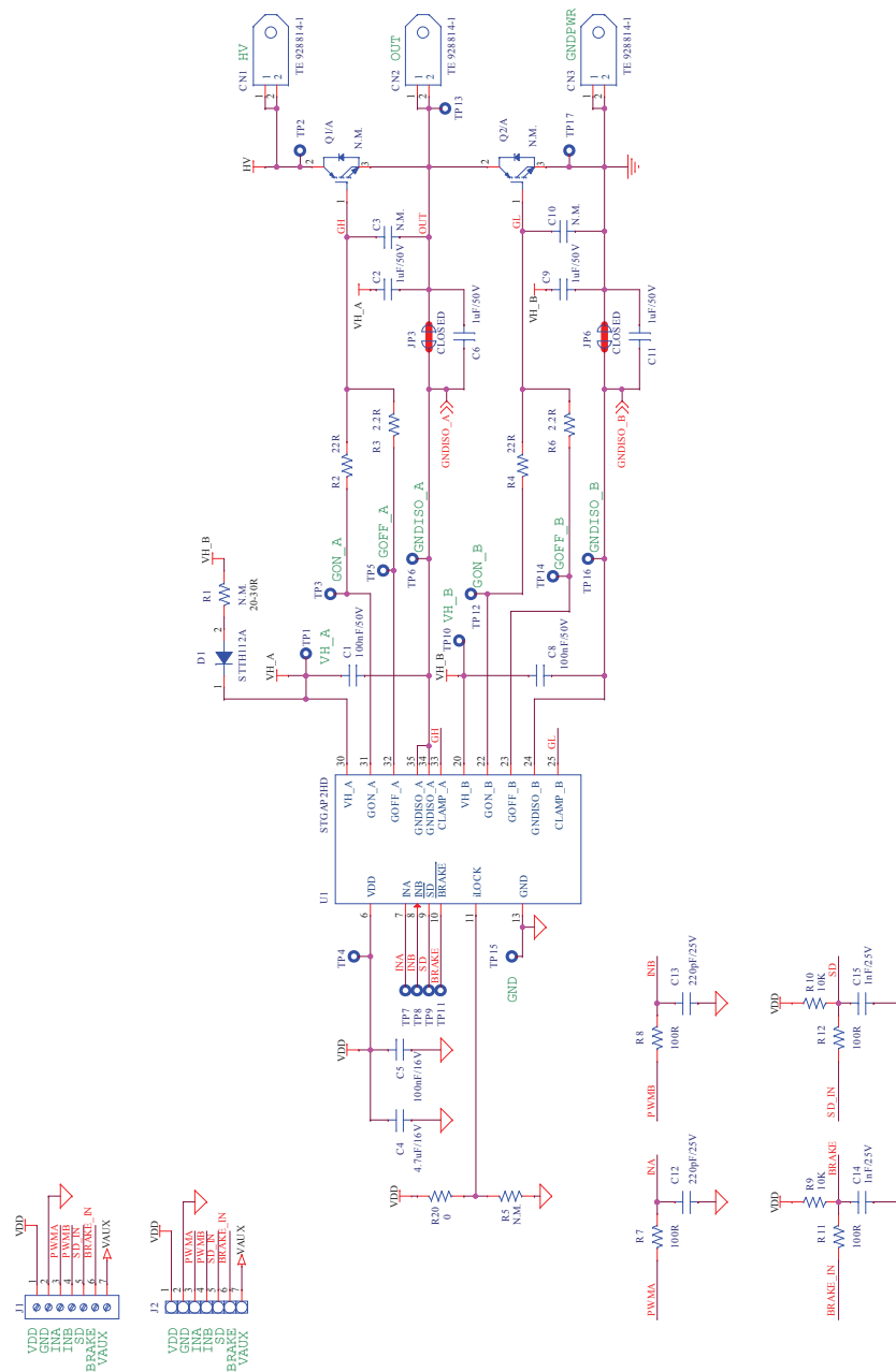
Figure 1. EVALSTGAP2HDM schematic – gate driver
