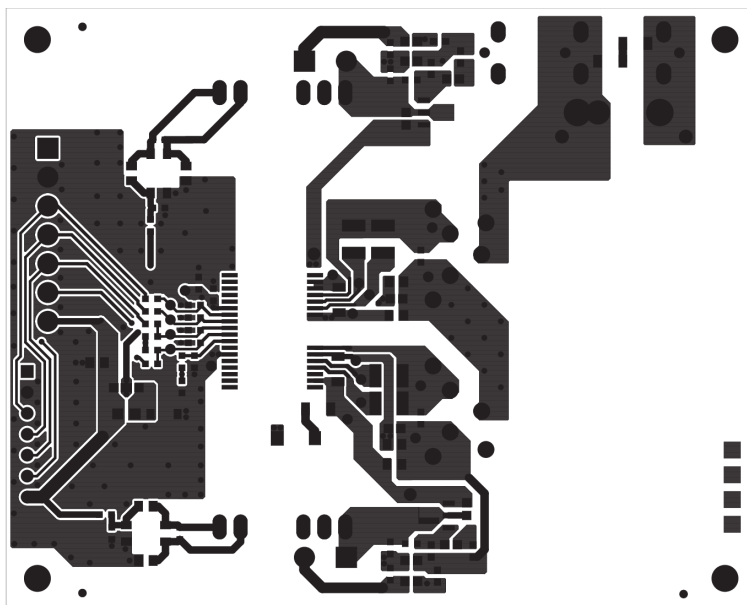
Figure 5. EVALSTGAP2HDM – Layout (top layer)
