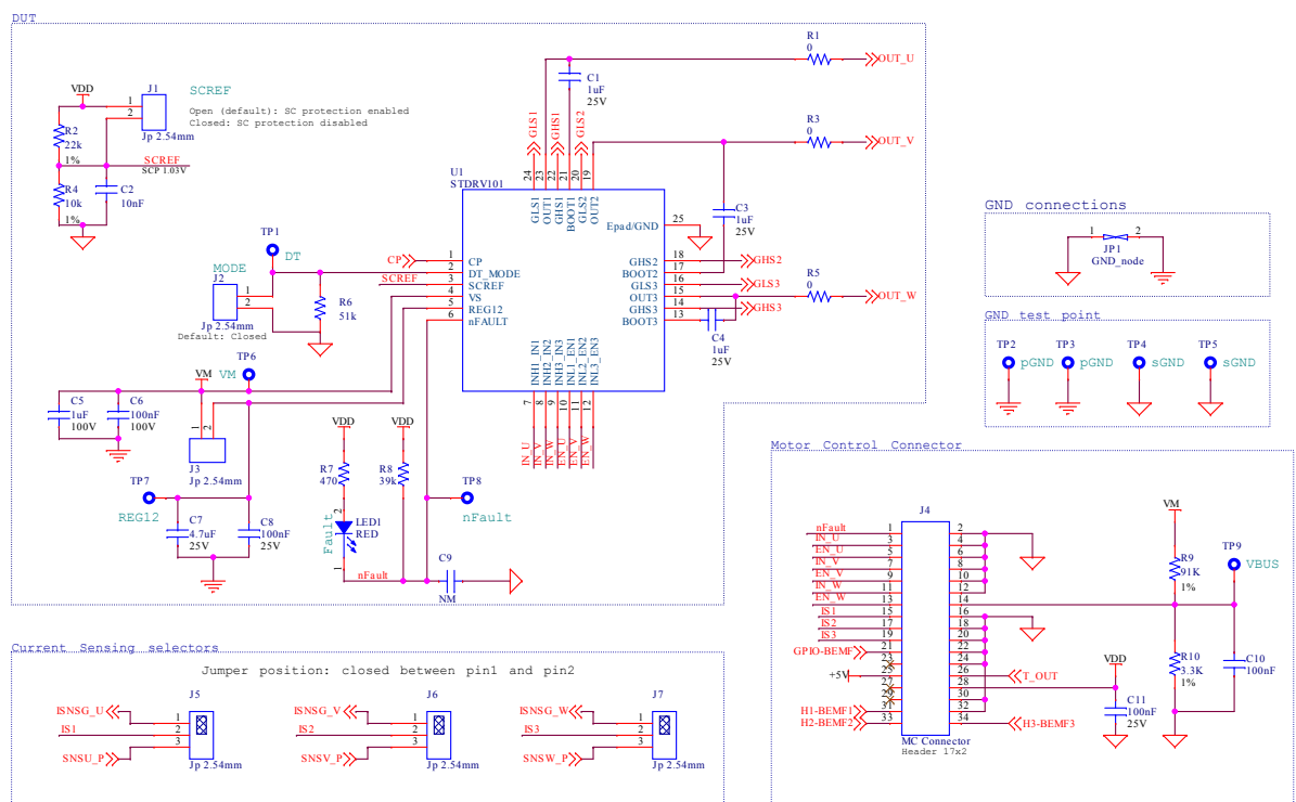
Figure 1. EVALSTDRI101 Schematic – Driver and MC connector
