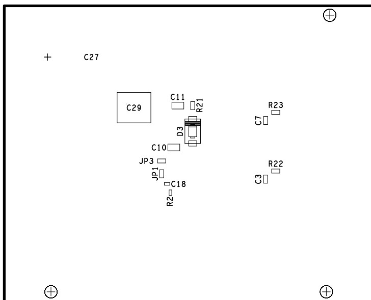
Figure 2. EVALMASTERGAN4 – bottom component placement
