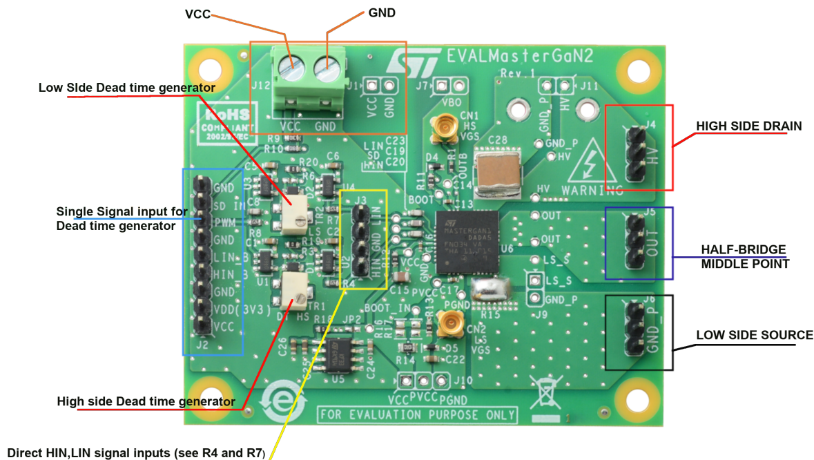
Figure 3. EVALMASTERGAN2 – Supply and signal connection
