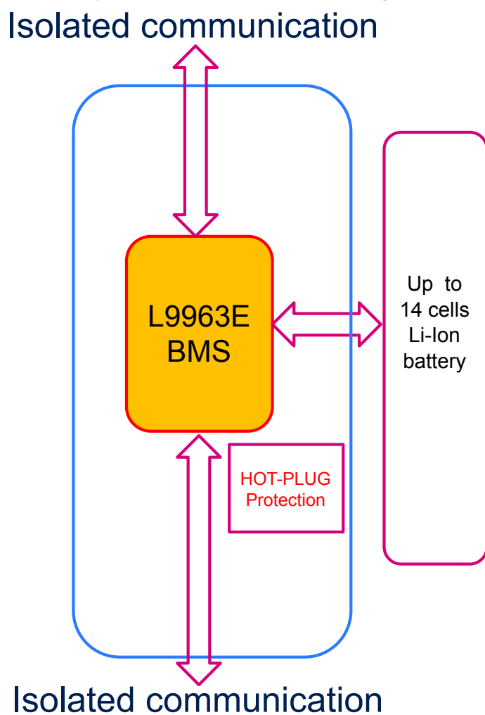
Figure 1. EVAL-L9963E-NDS block diagram
