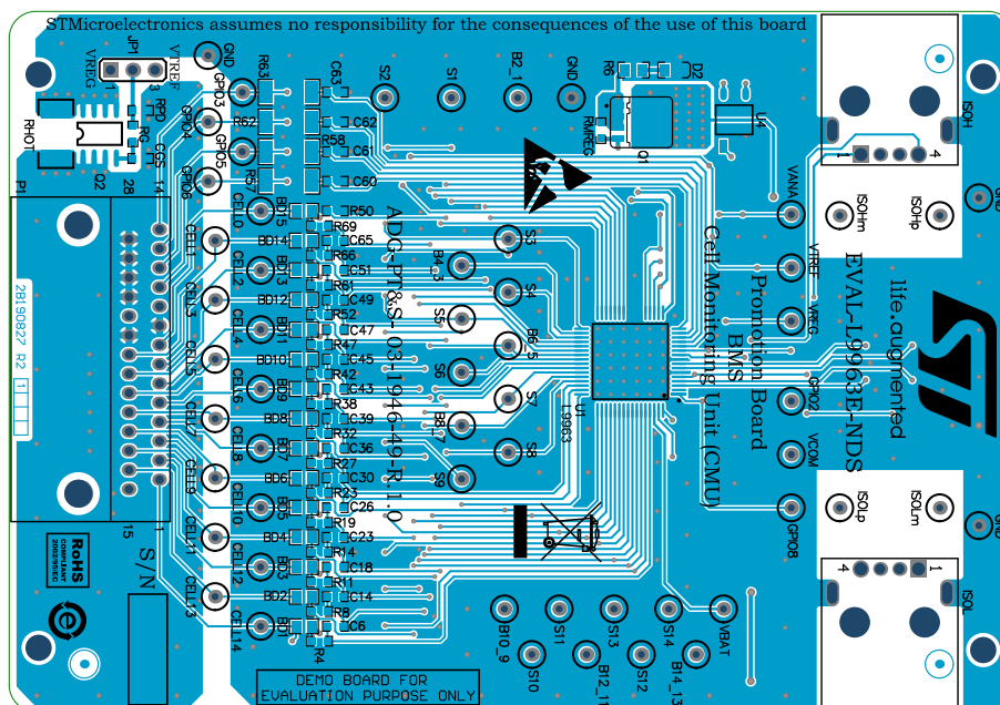
Figure 5. Assembly TOP
