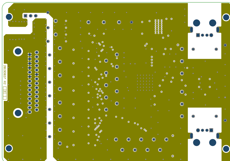
Figure 6. Inner 1
