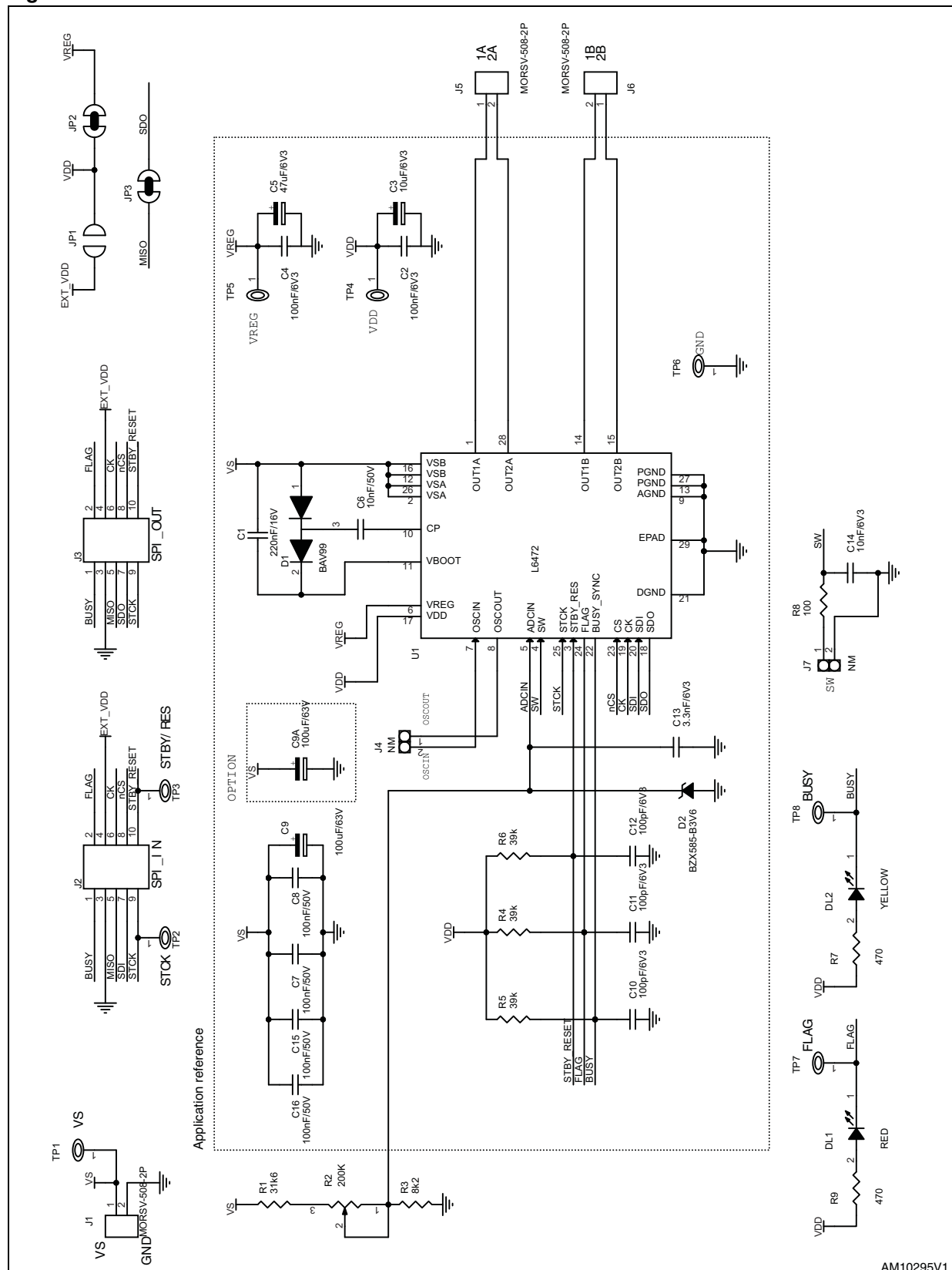
Figure 2. EVAL6472H schematic
