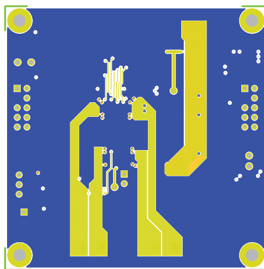
Figure 4. EVAL6470PD - layout (inner layer 2)
