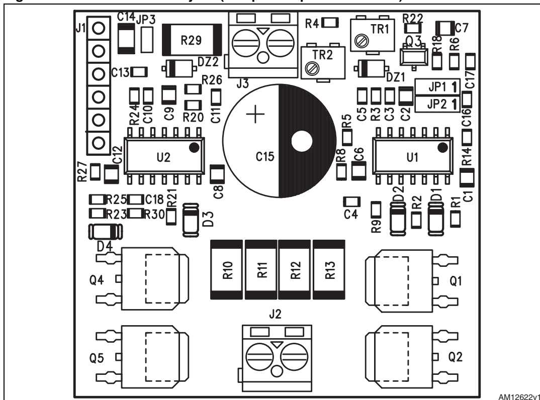
Figure 5. EVAL6393FB – layout (component placement view)
