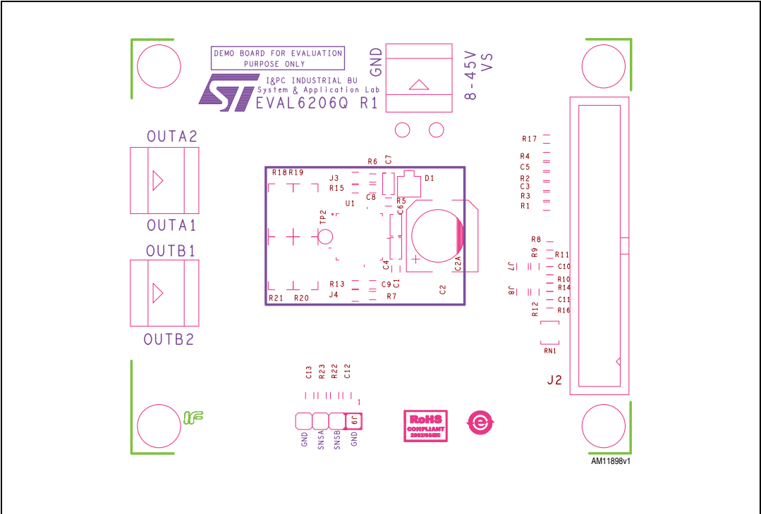
Figure 3. Layout (silk screen)
