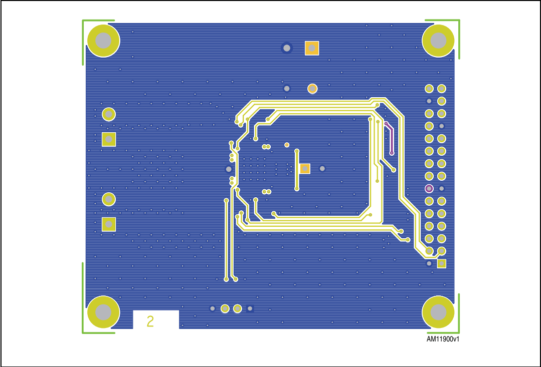
Figure 5. Layout (inner layer 2)
