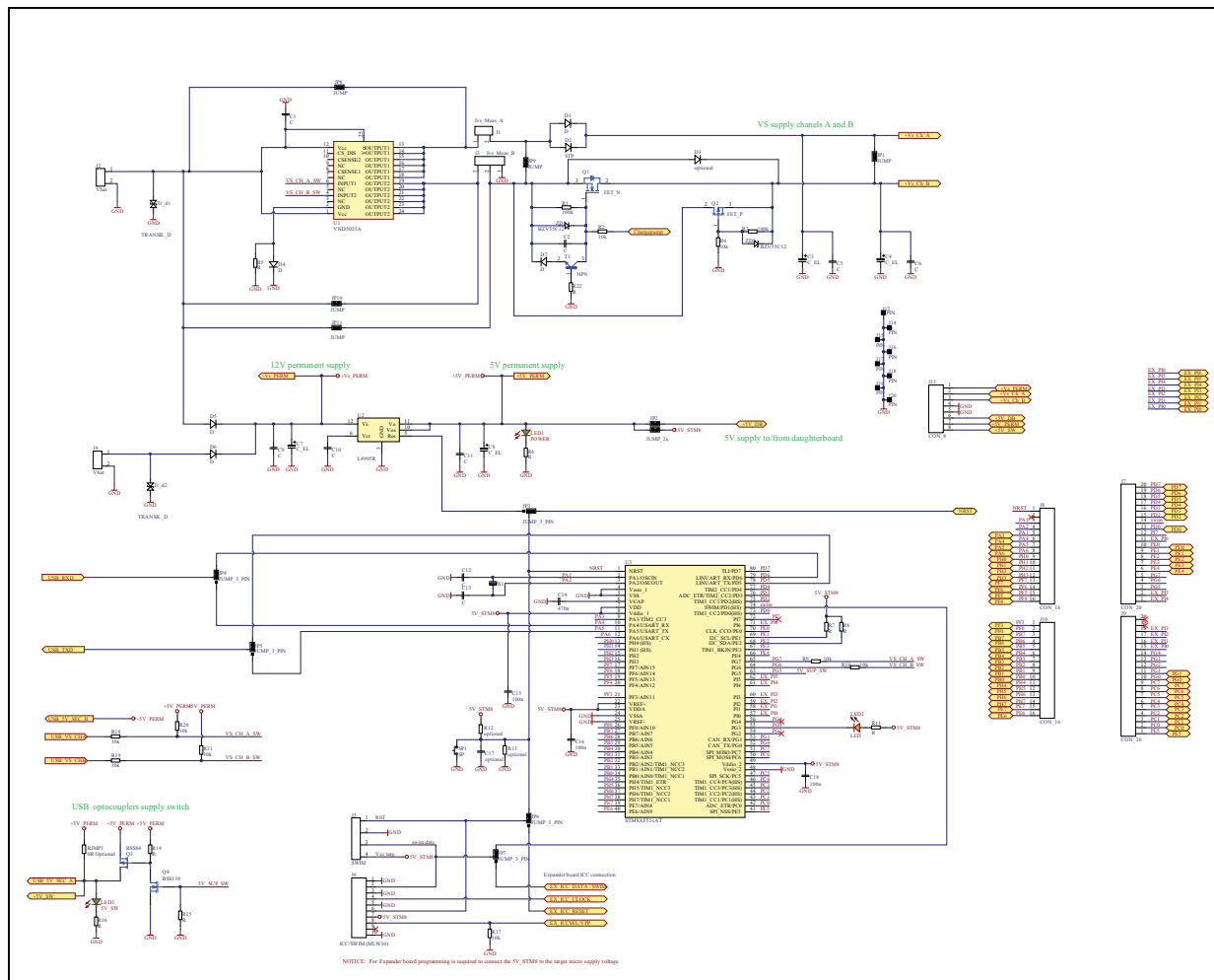
Figure 7. STM8 motherboard – STM8 &amp; Supply application schematic
