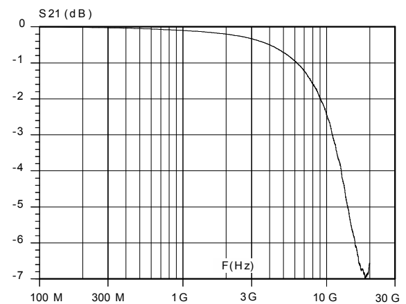
Figure 5. S21 attenuation
