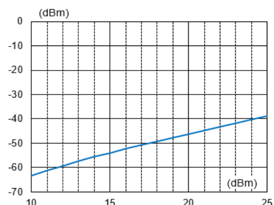
Figure 11. H3 harmonic versus input power at 824 MHz
