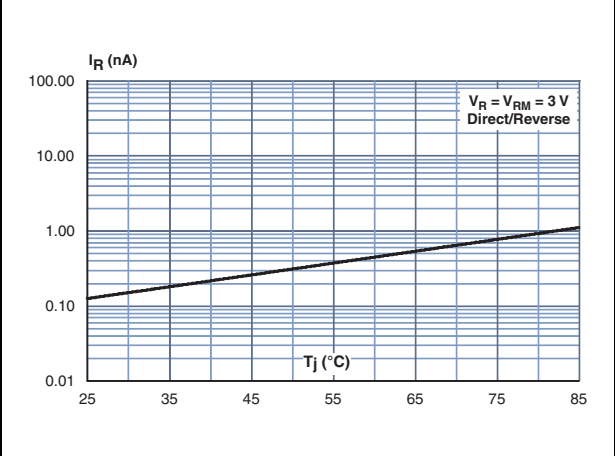
Figure 8. Leakage current versus junction temperature (typical values)
