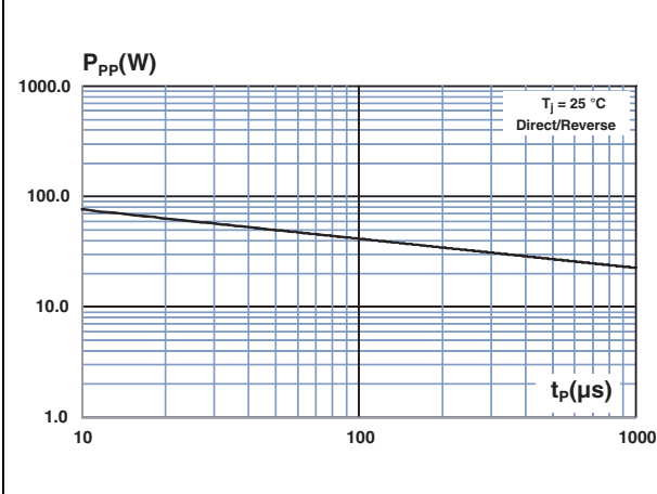
Figure 7. Peak pulse power versus exponential pulse duration
