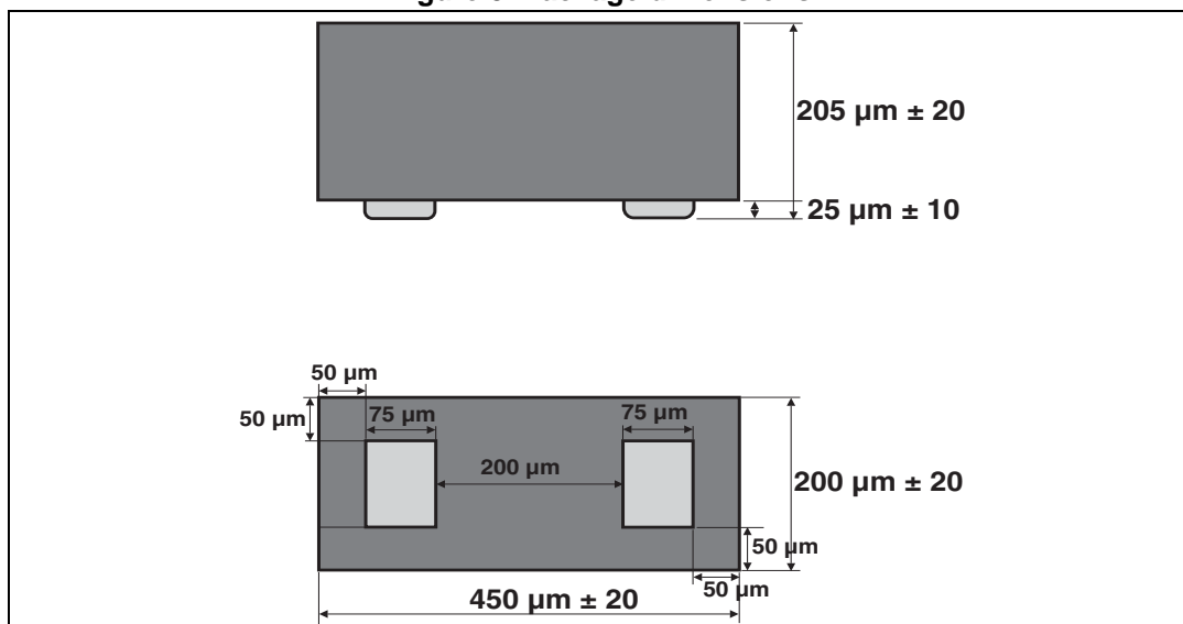
Figure 8. Package dimensions
