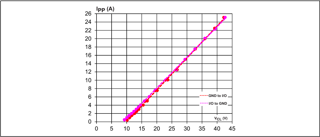
Figure 7. TLP measurement
