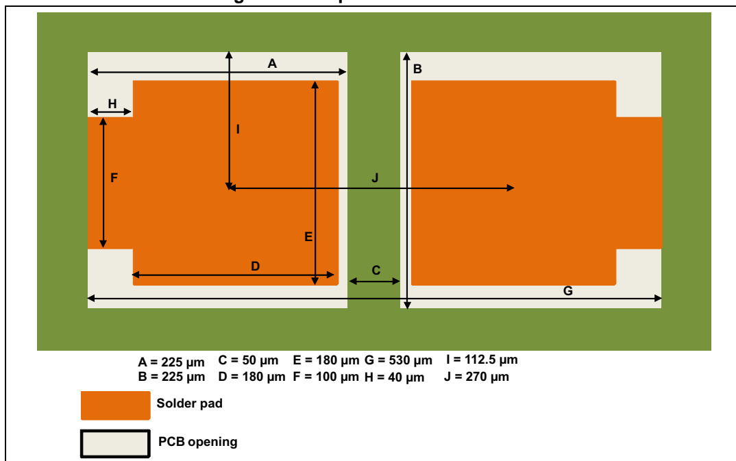
Figure 9. Footprint recommendation
