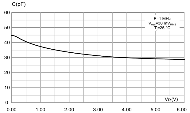
Figure 3. Junction capacitance versus applied voltage (typical values)
