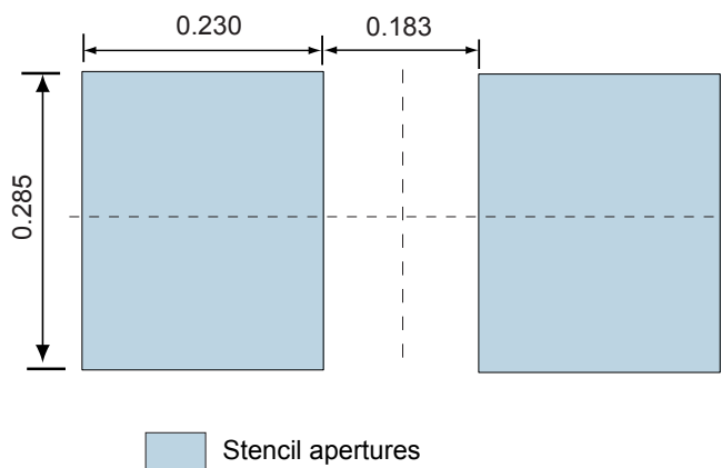
Figure 12. Stencil opening recommendations
