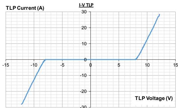
Figure 6. TLP
