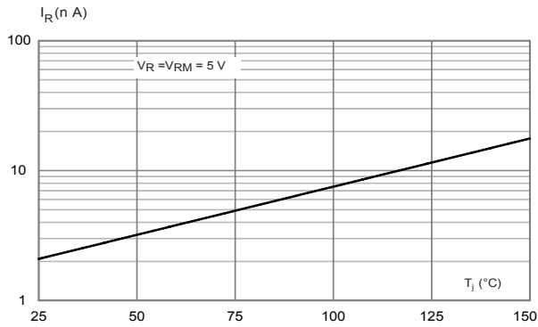
Figure 2. Variation of leakage current versus junction temperature
