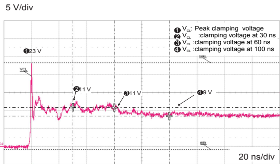
Figure 4. ESD response to IEC 61000-4-2 (+8 kV contact discharge)
