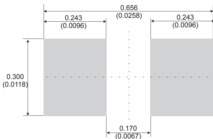
Figure 11. Footprint in mm
