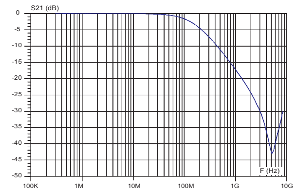
Figure 7. S21 attenuation
