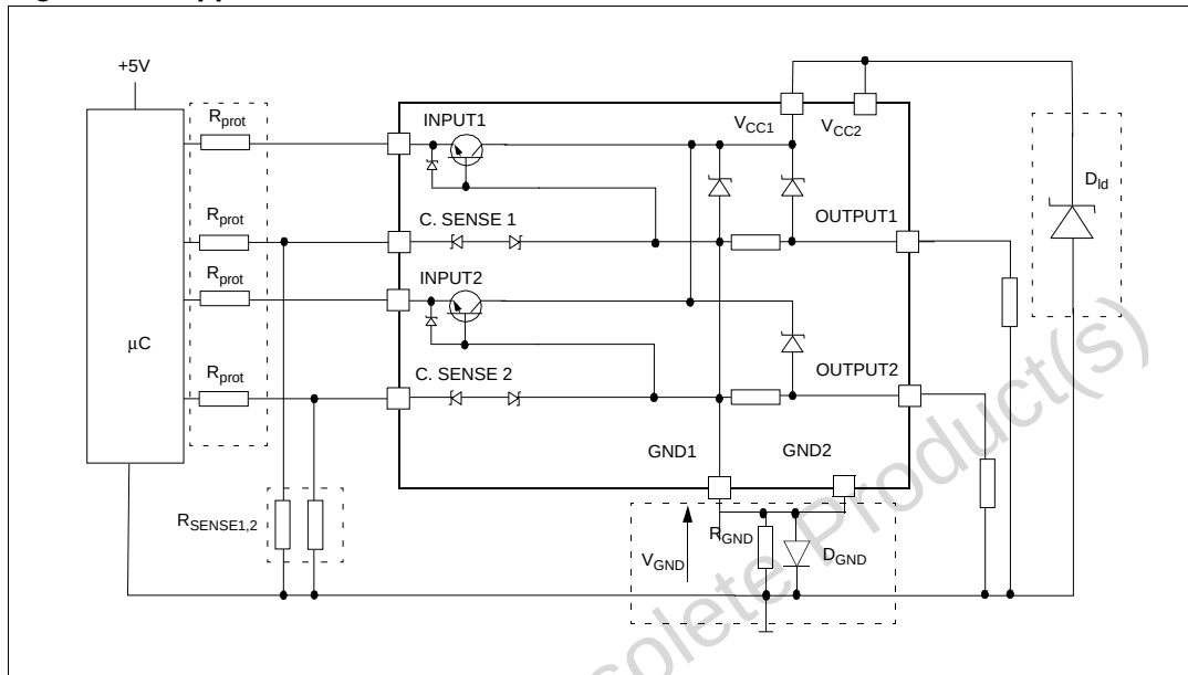
Figure 19. Application schematic
