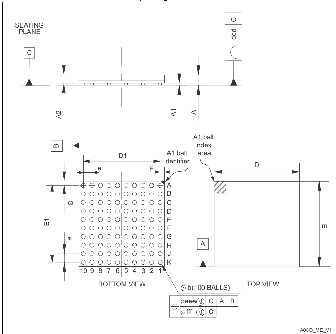
Figure 68. TFBGA100, 8 × 8 × 0.8 mm thin fine-pitch ball grid array package outline
