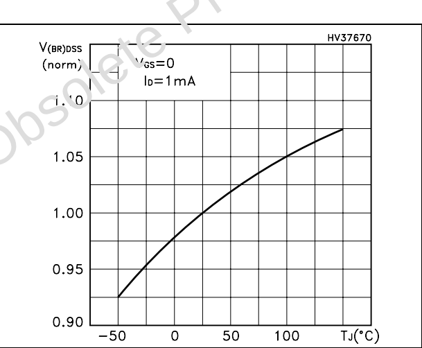
Figure 17. Normalized V_{(BR)DSS} vs temperature
