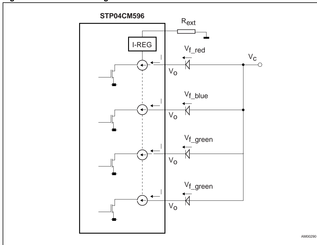
Figure 7. RGB LED configuration
