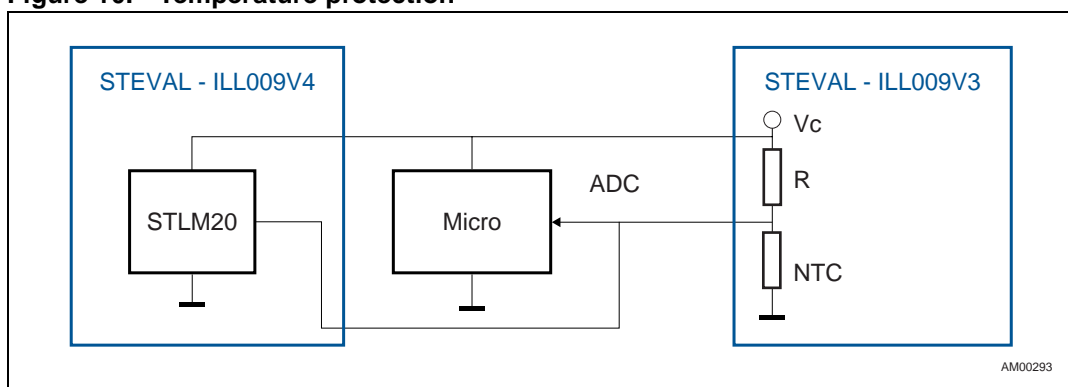
Figure 10. Temperature protection
