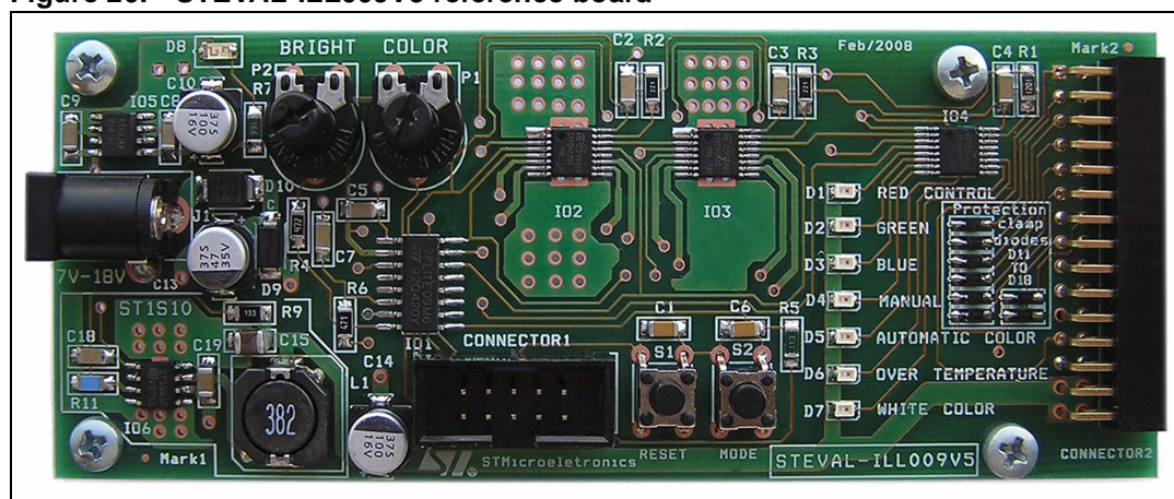
Figure 20. STEVAL-ILL009V5 reference board
