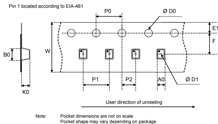
Figure 21. Tape and reel outline
