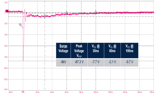
Figure 15. ESD response to IEC61000-4-2 (-8 kV contact discharge)
