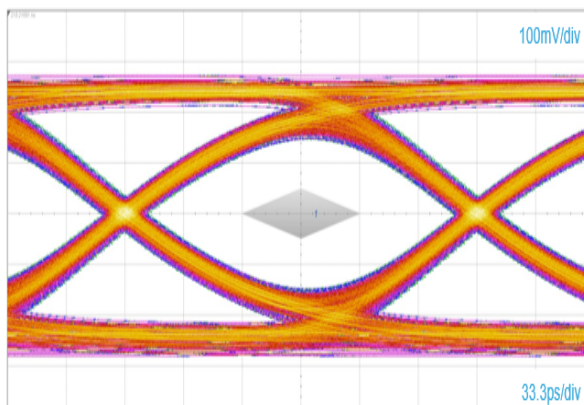
Figure 13. USB3.2 Gen 1 5.0 Gbps eye diagram with ECMFx-40A100Nx (with type C connector, reference cable and equalizer)
