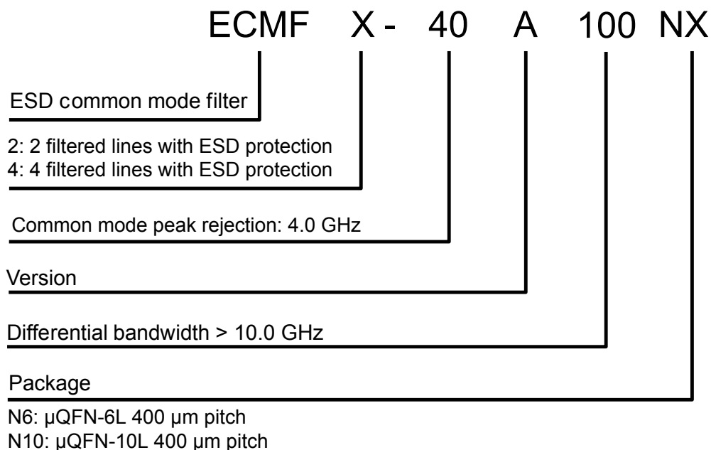
Figure 27. Ordering information scheme
