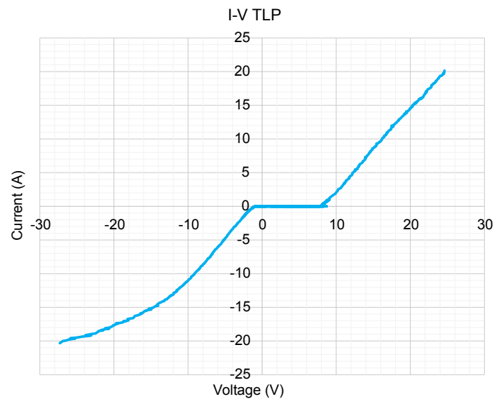
Figure 16. TLP characteristic
