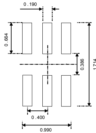
Figure 24. ECMF2-40A100N6 stencil opening recommendations
