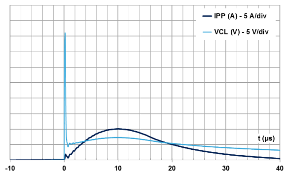
Figure 7: Clamping response to 8/20 \mu s surge ( I_{pp} = 10 A )
