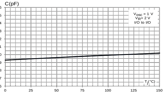
Figure 6: Junction capacitance versus junction temperature
