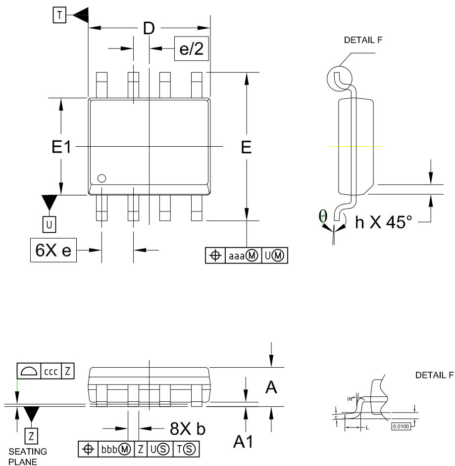
Figure 14. SO-8 mechanical data
