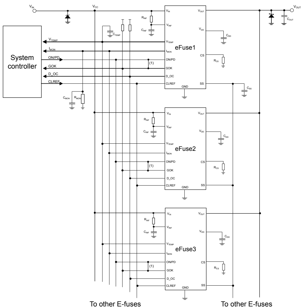
Figure 5. Typical application diagram (multiple e-fuses in parallel)
