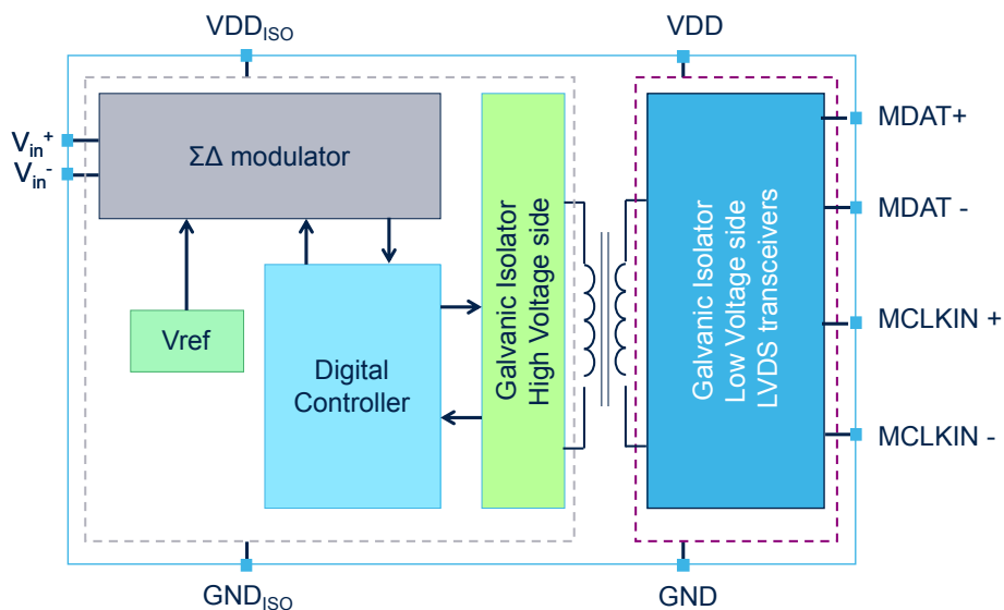
Figure 1. ISOSD61L Block diagram
