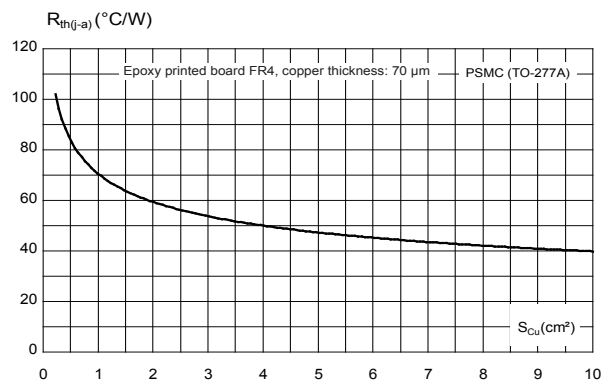
Figure 6. Thermal resistance junction to ambient versus copper surface under tab (typical values, epoxy printed board FR4, e_{Cu} = 70 \mu m ) (PSMC (TO-277A))
