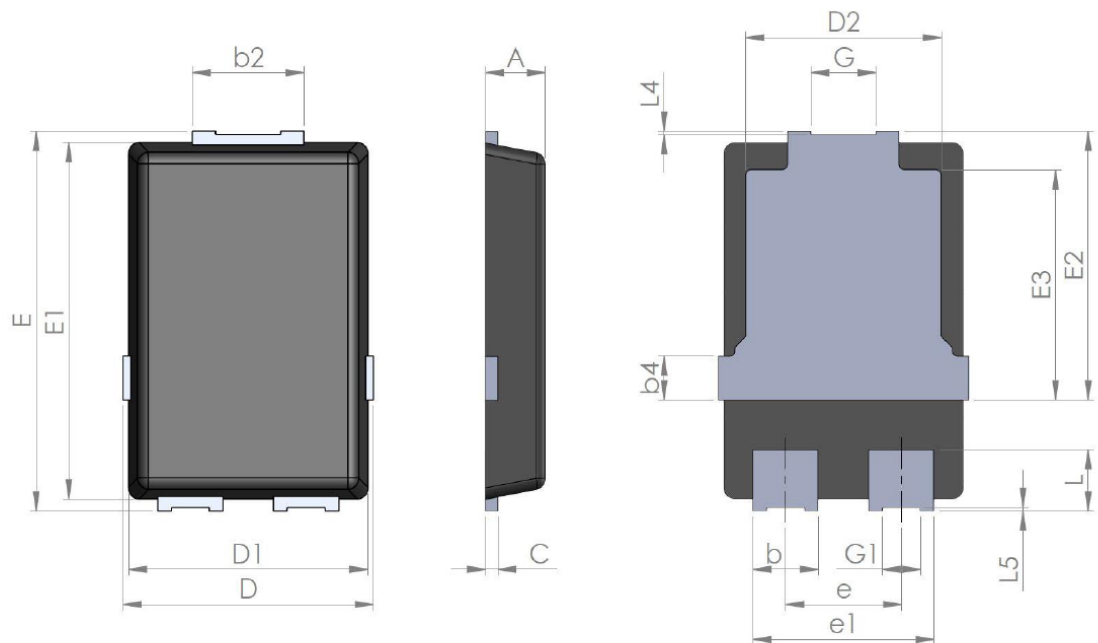
Figure 7. PSMC (TO-277A) package outline
