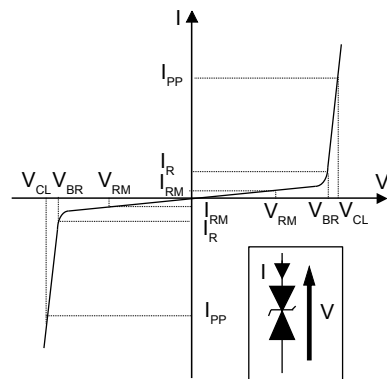
Figure 1. Electrical characteristics (definitions)
