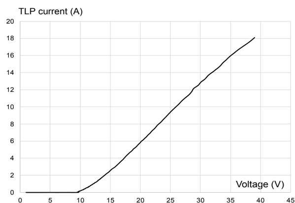
Figure 9. Negative TLP characteristic
