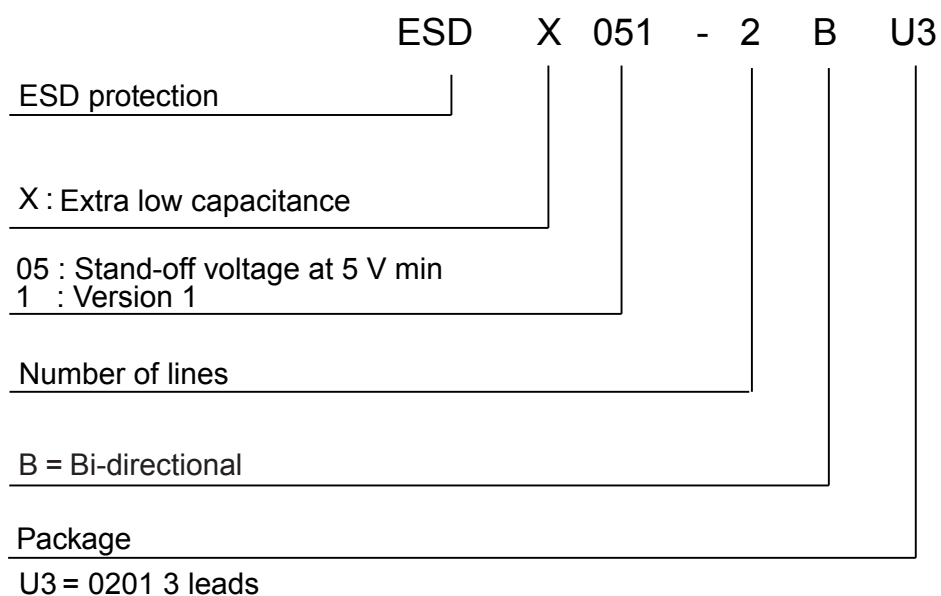
Figure 16. Ordering information scheme
