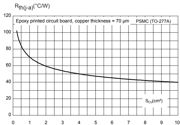
Figure 11. Thermal resistance junction to ambient versus copper surface under tab (typical values, epoxy printed board FR4, e_{Cu} = 70\text{ }\mu\text{m} ) (PSMC (TO-277A))
