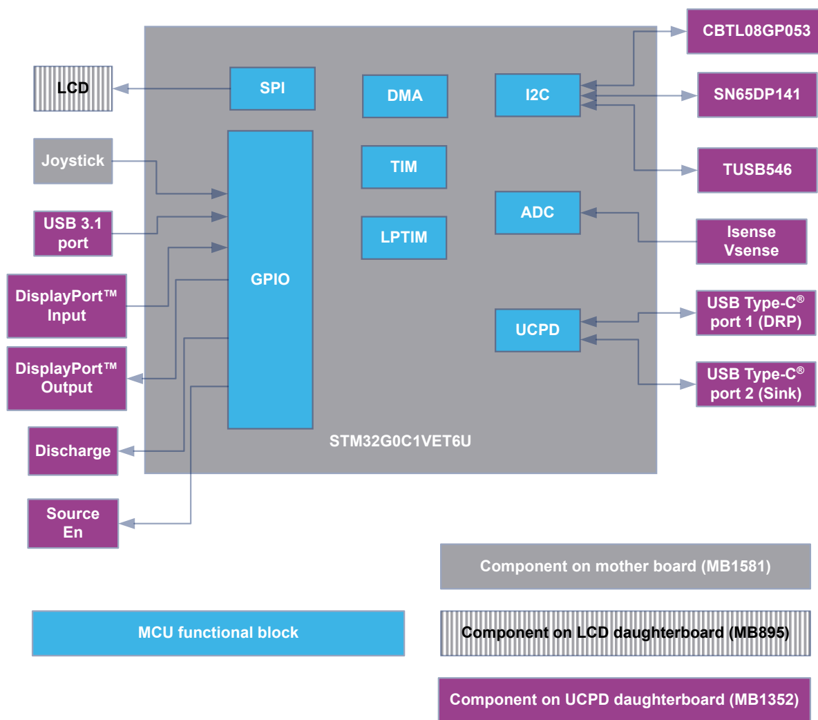
Figure 12. STM32G0C1VET6 peripherals used by the UCPD application
