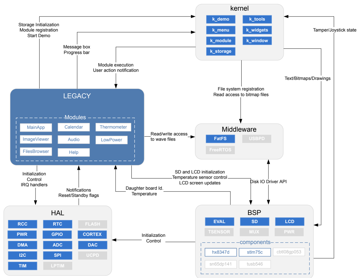
Figure 61. Legacy application software architecture block diagram
