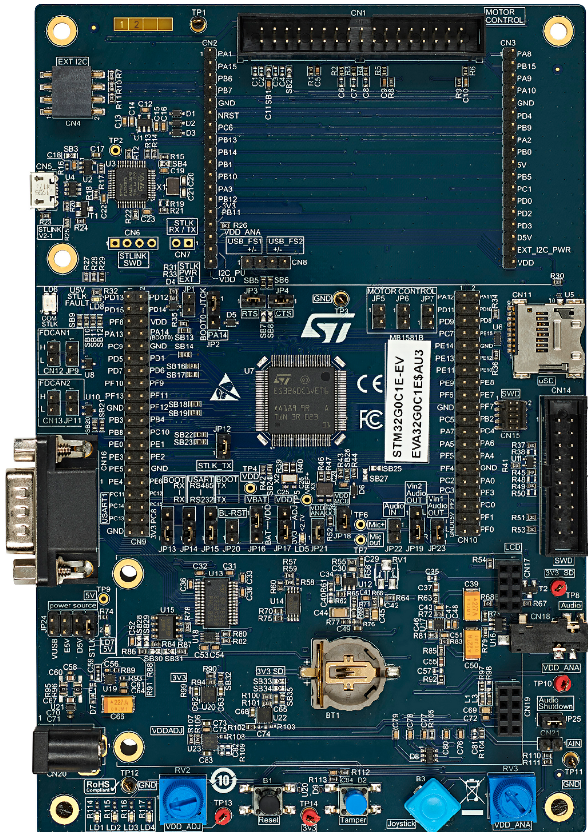
Figure 4. STM32G0C1E-EV Evaluation board (MB1581)
