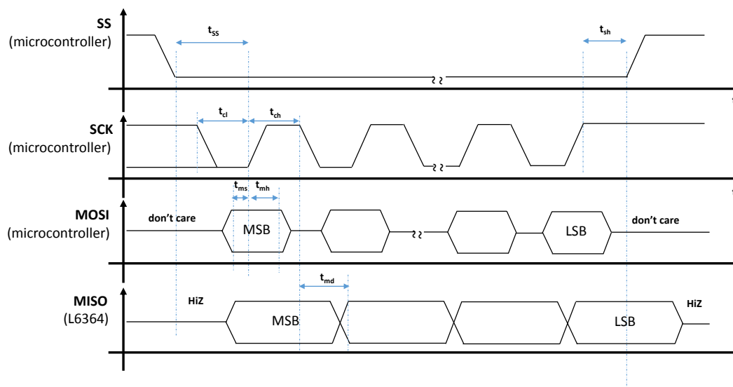
Figure 5. Register programming.
