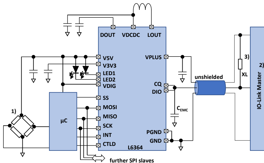
Figure 22. Application example: DC-DC enabled, CQ and DIO coupled (Join Mode), V_{\text{SENSOR}} = V_{\text{MCU}} = \text{VDIG} = 5.0\text{ V}
