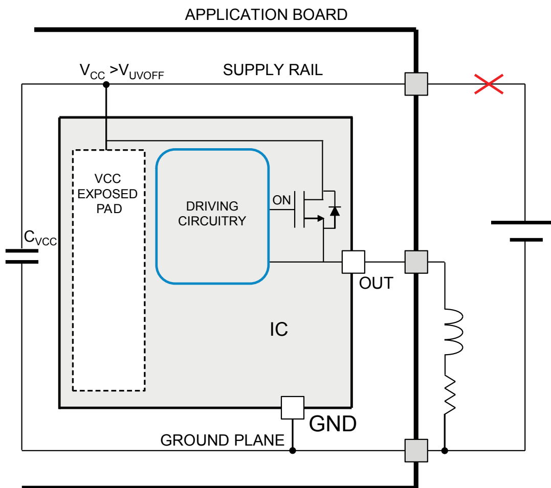
Figure 8. VCC disconnection
