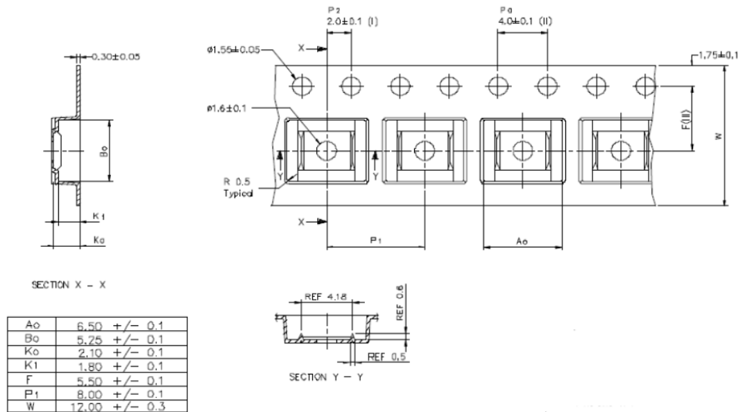
Figure 16. PowerSSO12 reel packing information [mm]
