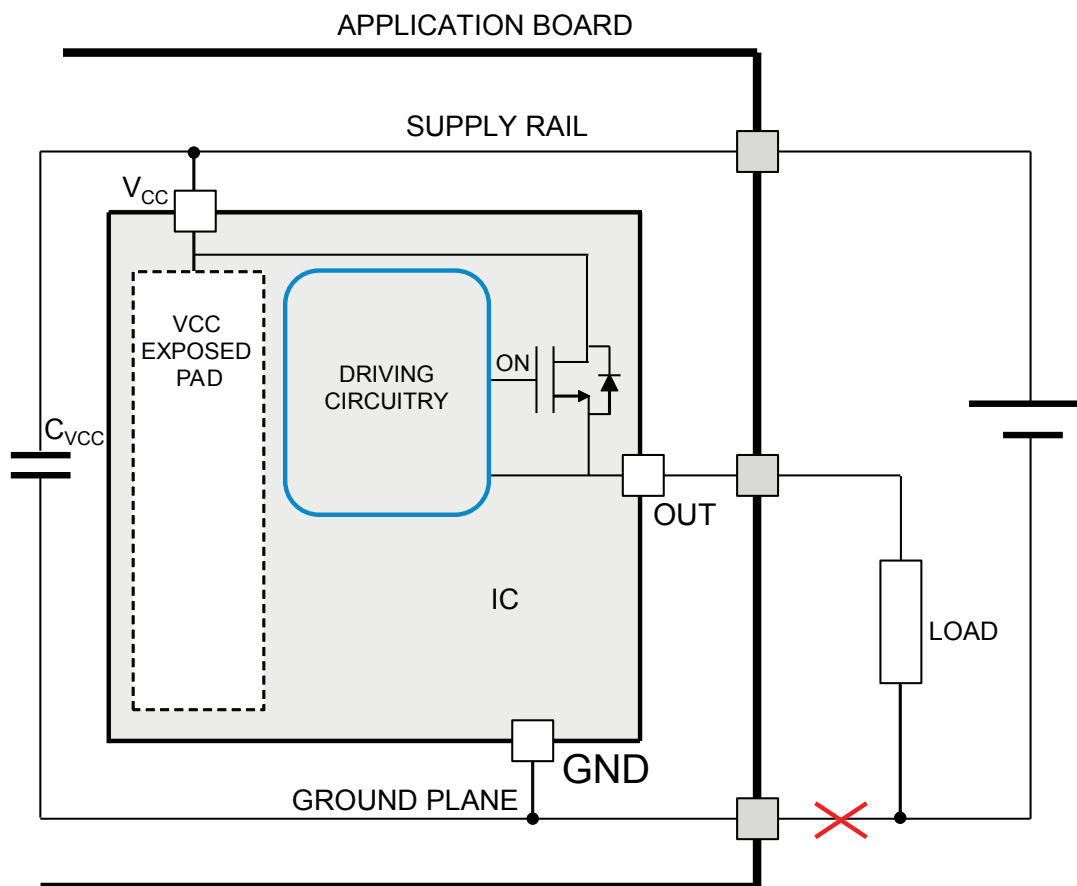
Figure 9. GND disconnection
