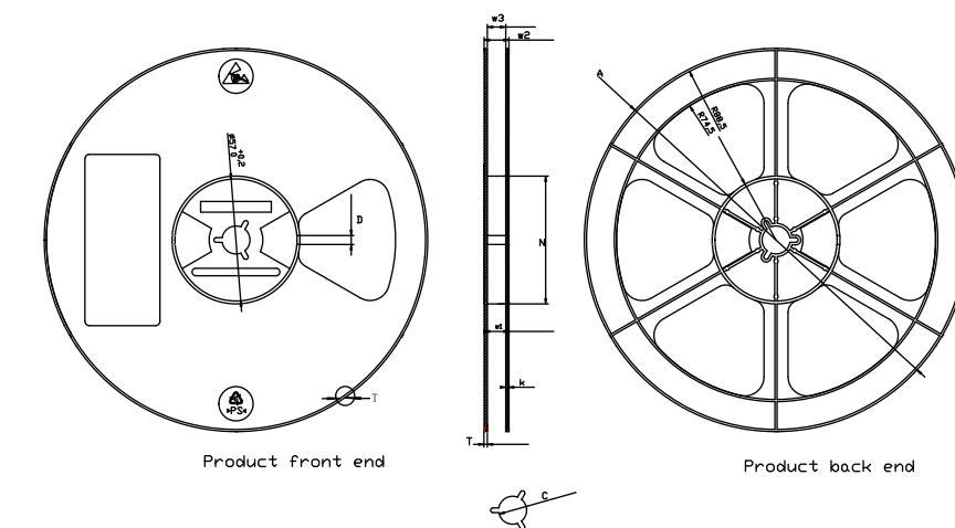
Figure 31. TQFN12 (2.0x1.70x0.55 mm) reel outline
