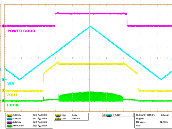
Figure 9. 100% mode, V_{OUT} = 2.5\text{ V} , 50 mA load
