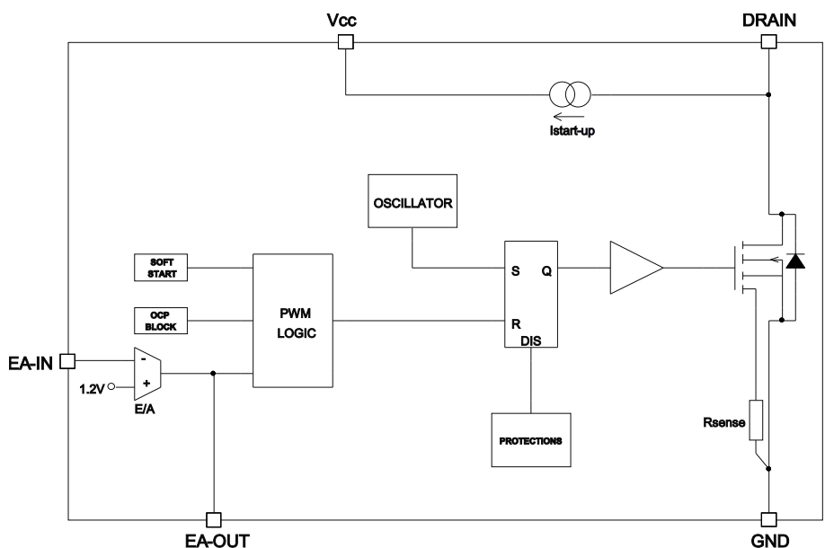
Figure 1. Block diagram
