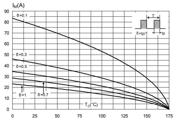
Figure 4. Peak forward current versus case temperature (fw > 10 kHz)
