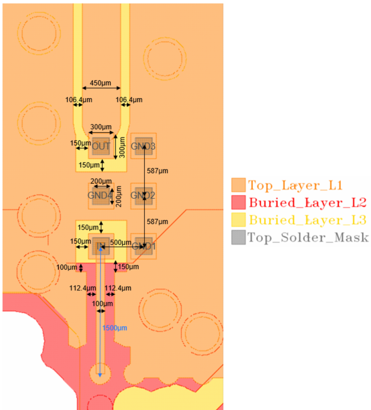
Figure 13. PCB land pattern recommendations
