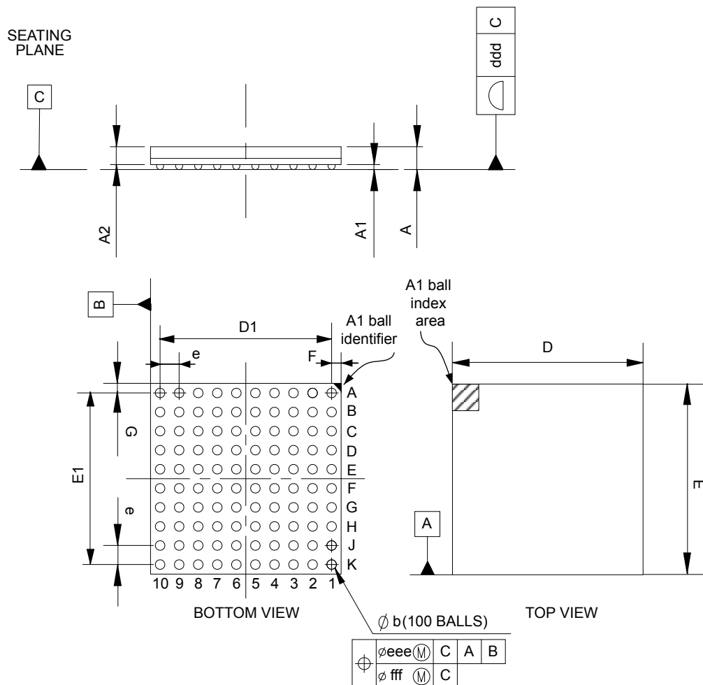
Figure 88. TFBGA100 - Outline
