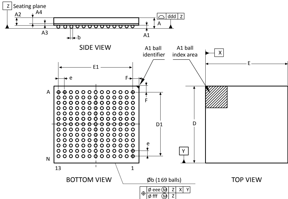
Figure 106. UFBGA169 - Outline
