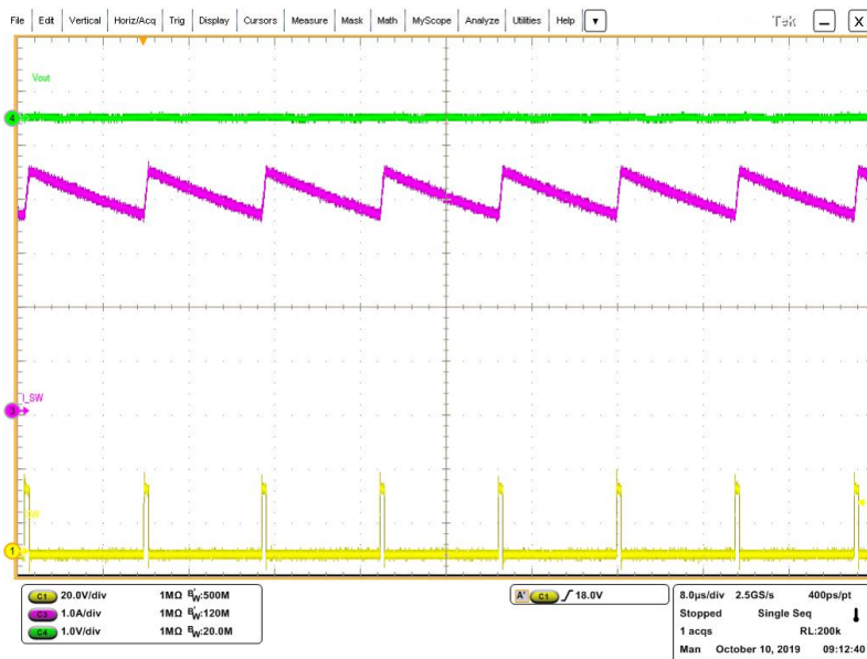
Figure 21. Over current procedure with persistent short circuit between V_{OUT} and GND
