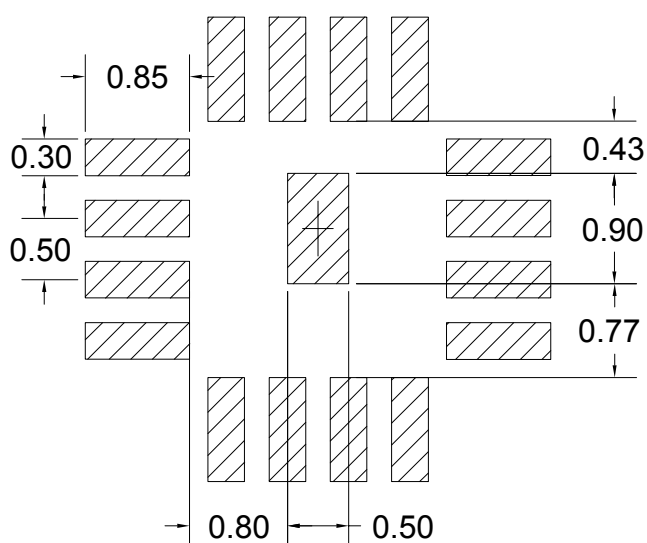
Figure 59. QFN16 (3x3 mm) recommended footprint
