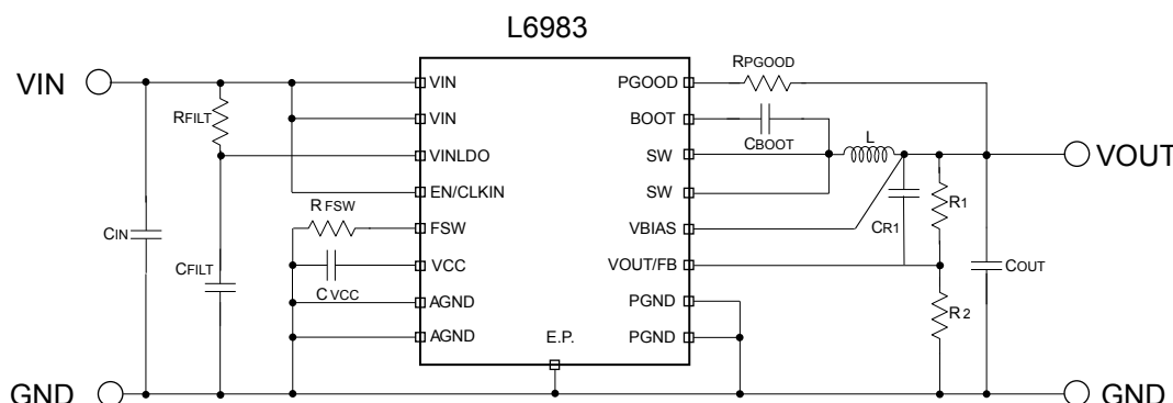
Figure 29. Application circuit
