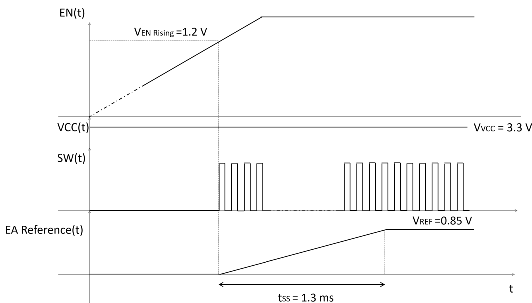
Figure 5. Soft-start procedure
