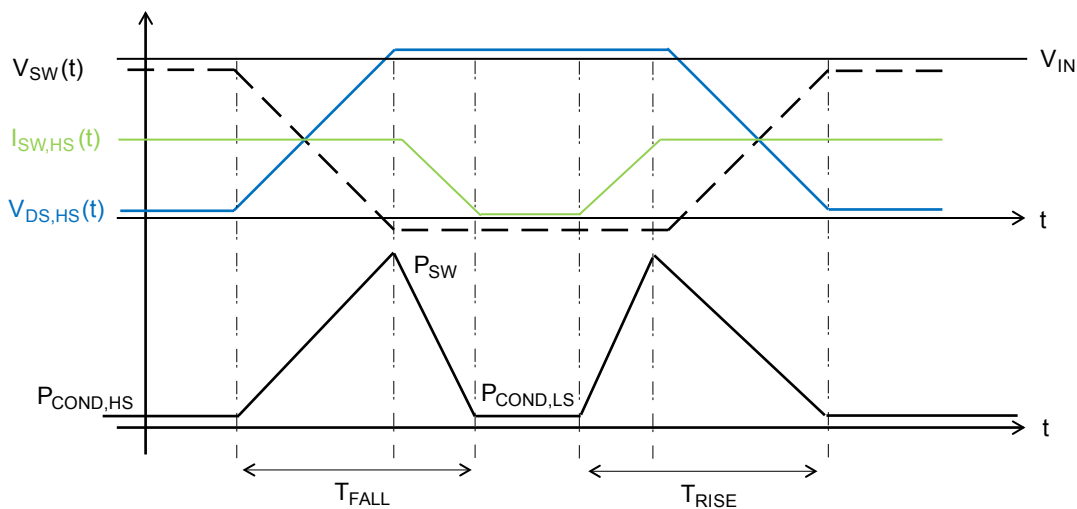
Figure 57. Switching losses
