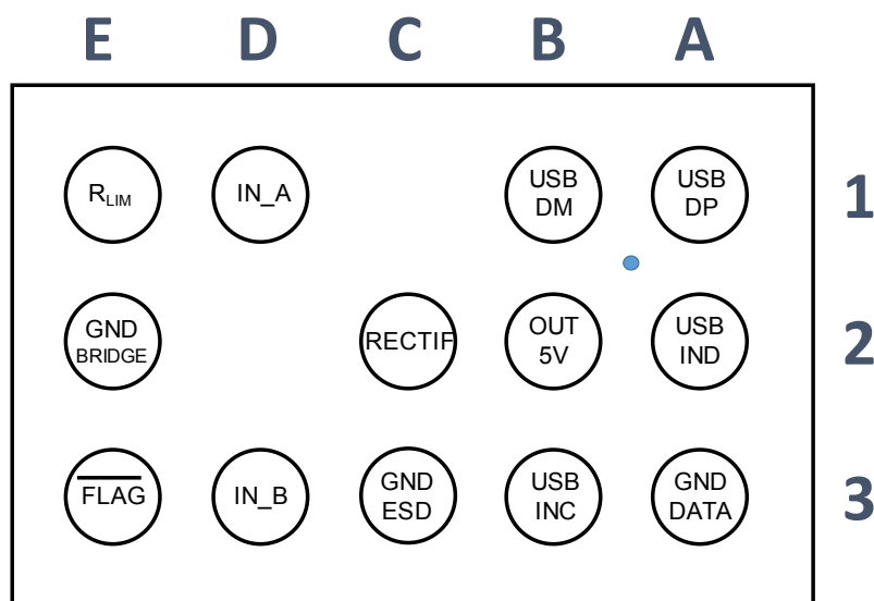
Figure 3. Pin numbering (bump side)
