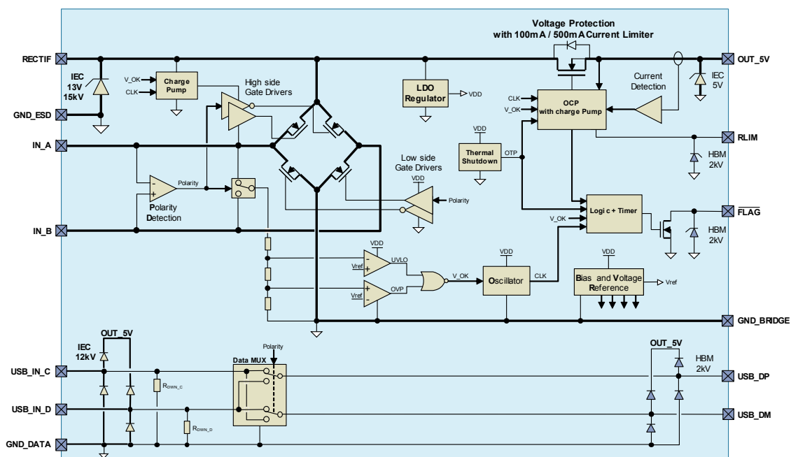
Figure 2. Functional diagram
