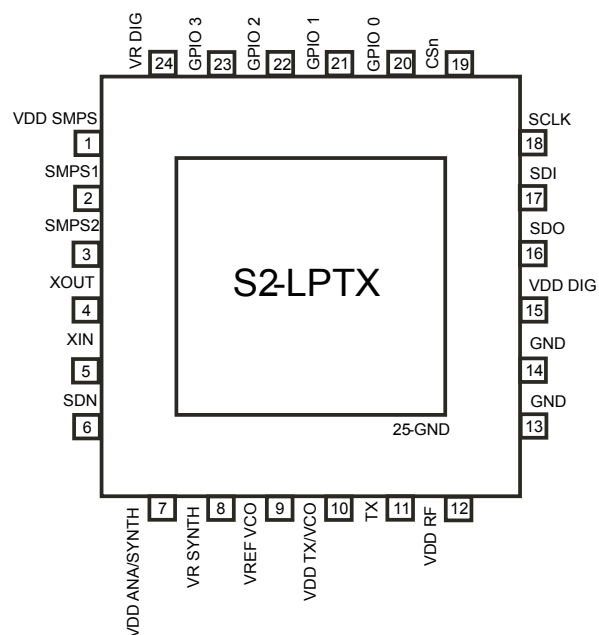
Figure 5. Pin diagram, QFN24 (4x4 mm) package
