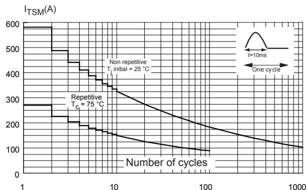
Figure 5. Surge peak on-state current versus number of cycles ( V_R = 0 V)
