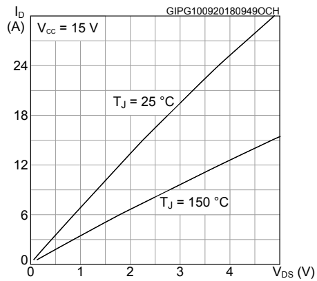
Figure 9. Output characteristics
