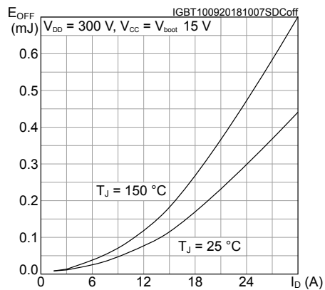
Figure 13. E_{OFF} switching energy vs drain current
