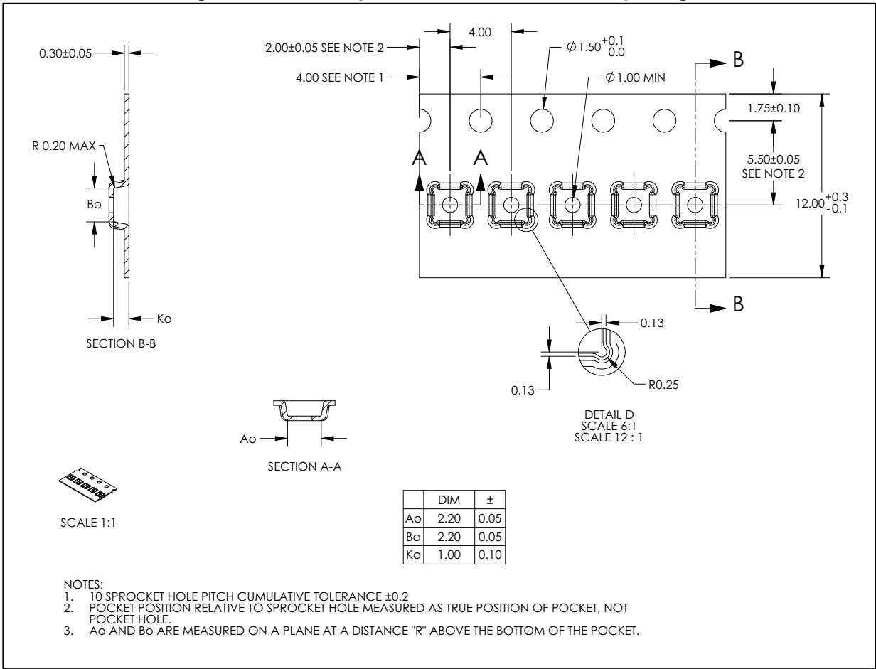
Figure 25. Carrier tape information for HLGA-10L package
