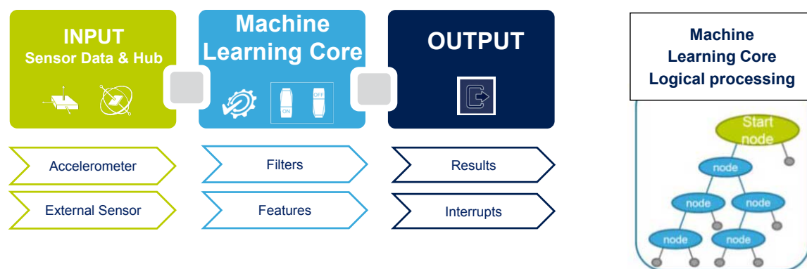
Figure 3. Machine Learning Core in the IIS2ICLX
