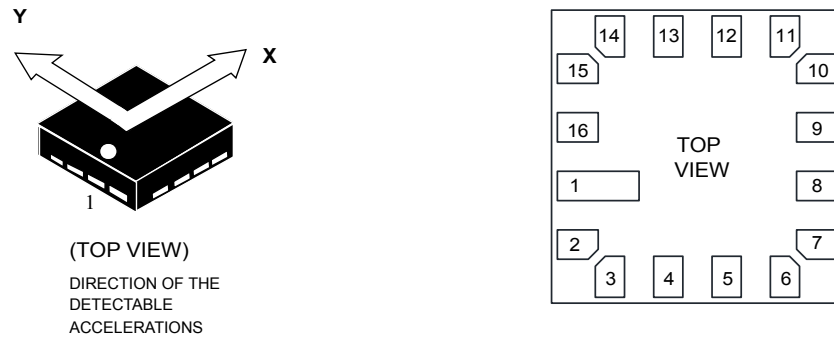
Figure 4. Pin connections
