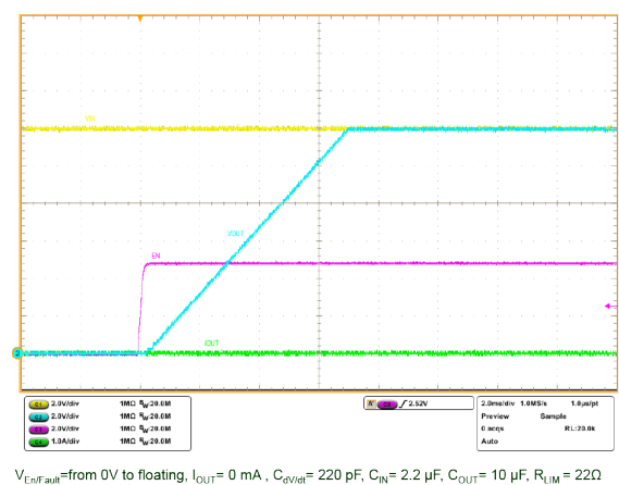
Figure 25. Start-up via En/Fault pin (no load)
