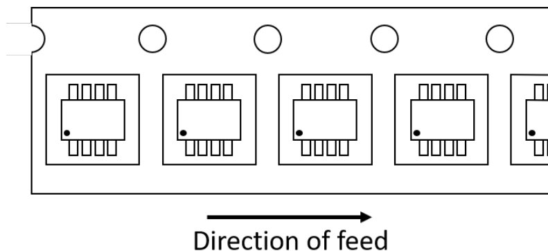
Figure 42. TSOT23-8L device orientation in tape
