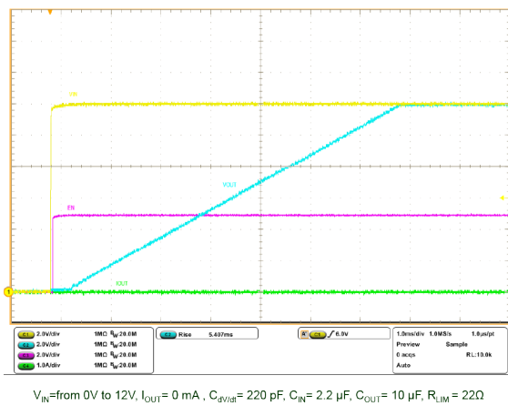
Figure 24. Start-up via input voltage (no load)
