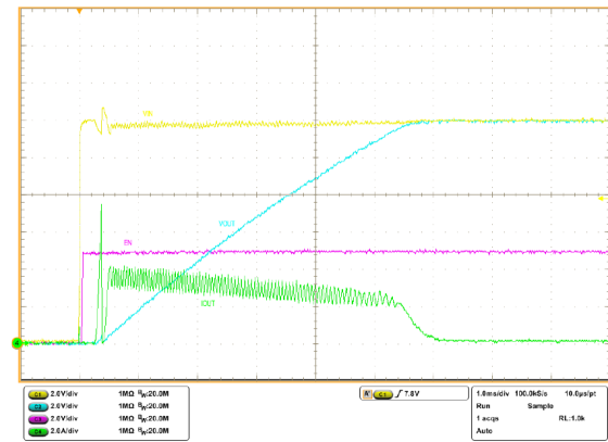
Figure 27. Start-up via input voltage ( C_{OUT} = 1500\ \mu\text{F} )
