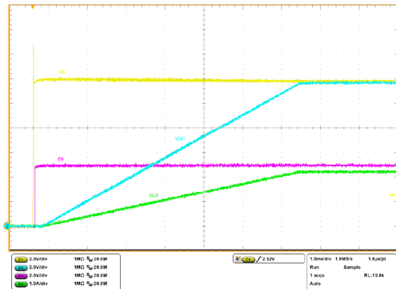
Figure 26. Start-up via input voltage (5 \Omega load)
