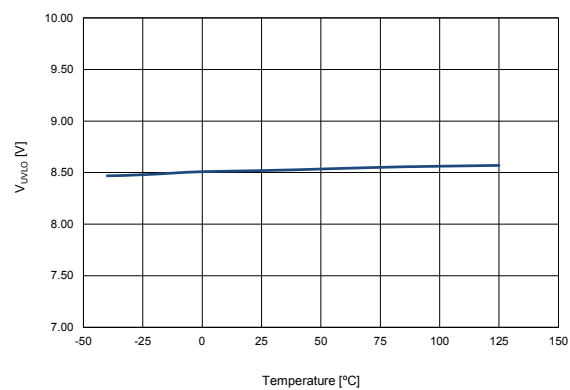
Figure 18. V_{UVLO} vs. temperature
