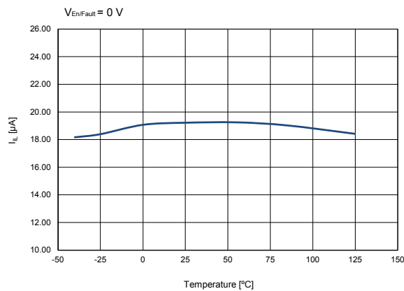
Figure 22. En/Fault pin current vs. temperature (En/Fault to GND)
